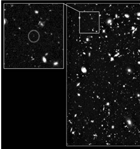
The circled image in the enlarged square of this Hubble Space Telescope Ultra Deep Field camera is the most distant galaxy yet discovered (as of 2011). Sixteen hours of follow-up observations measuring the redshift with the SINFONI spectrograph on the Very Large Telescope in Chile confirmed the galaxy, UDFy-38135539, to be 13.1 \times 10^9 c \cdot y from Earth, receding at about 0.97c , or about 30 \times 10^6 c \cdot y farther than the next most distant galaxy. The galaxy probably formed about 600 million years after the Big Bang. [M. Lehnert (Paris Observatory) et al., Nature , Oct. 21, 2010.]
